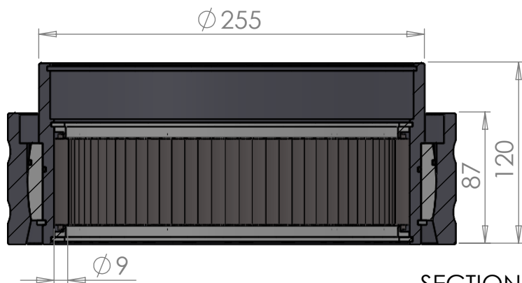
SECTION A-A SCALE 1 : 3.5
