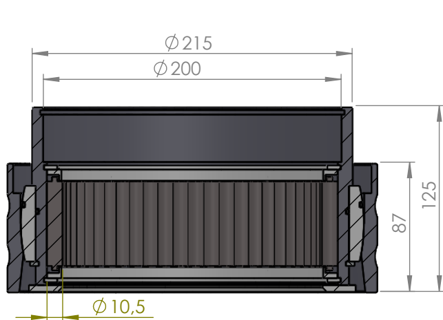
SECTION A-A SCALE 1 : 3.5
