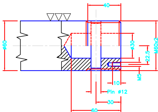
TOP SHAFT DETAIL
