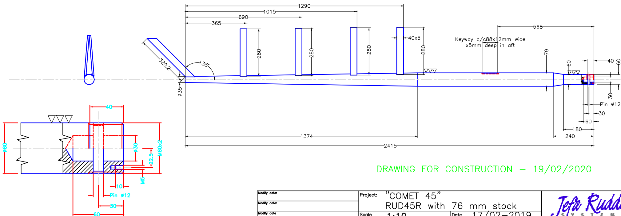
TOP SHAFT DETAIL
